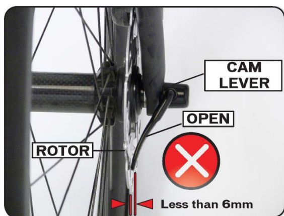
Figure 1. Quick-release lever with potential for contact Figure 2. Quick-release lever with adequate clearance
